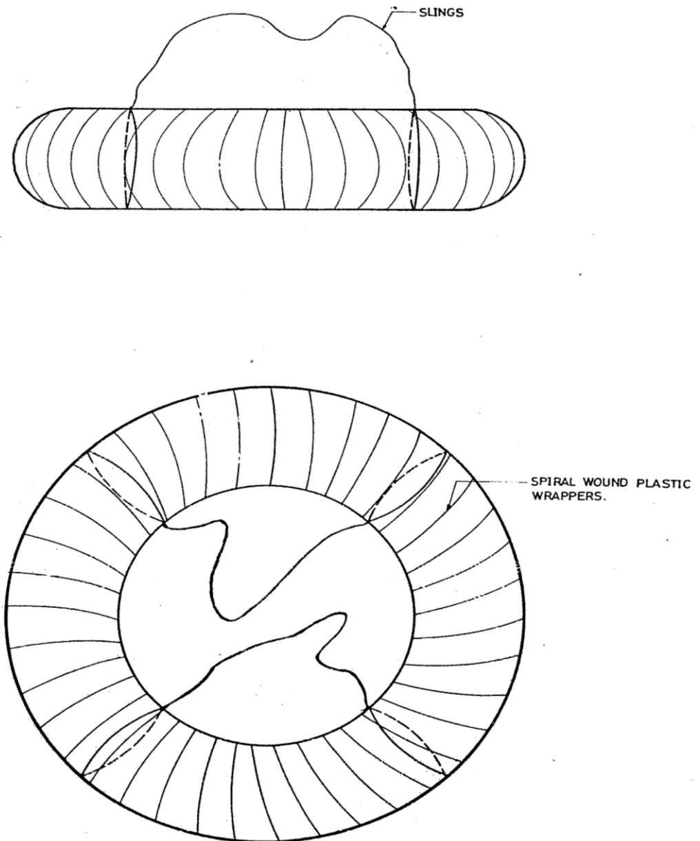
SLING ARRANGEMENT FOR LIFTING 63 mm \phi COILS
